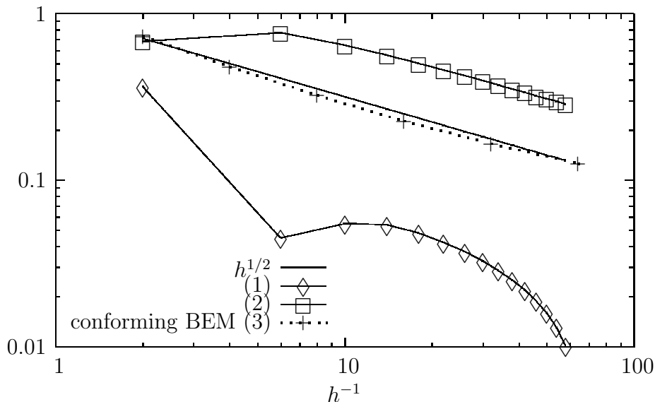
Figure 3: Relative error curves (normalised by \|u\|_{\text{ex}} ): (1) |\|u\|_{\text{ex}} - \langle f, u_h \rangle|^{1/2} , (2) h^{1/4} \left( \sum_{e \in \mathcal{E}_h} \|[u_h]\|_{0,e}^2 \right)^{1/4} , (3) error in \tilde{H}^{1/2}(\Gamma) for conforming BEM.
