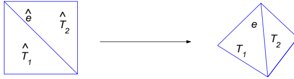
Figure 1: The reference double triangle of the proof of Proposition 6 and its transformed image.
