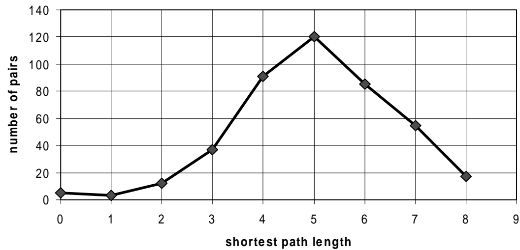
B Distribution of shortest path length between random pairs of enzymes
